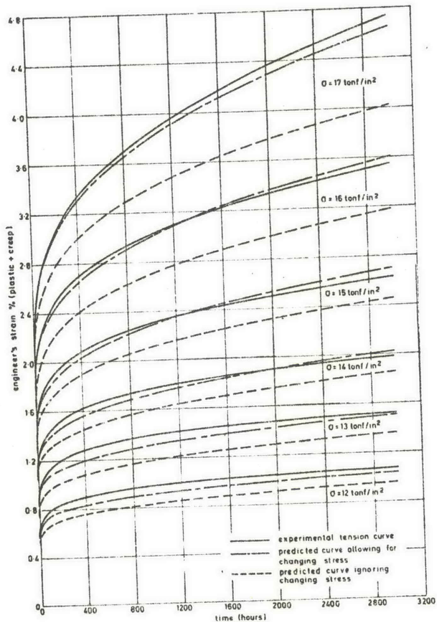
FIG. 13 COMPARISON OF EXPERIMENTAL TENSION CREEP CURVES WITH THOSE PREDICTED FROM TORSION CREEP DATA ON BASIS OF VON MISES FLOW RULE (0.18 PERCENT CARBON STEEL AT 400°C)
